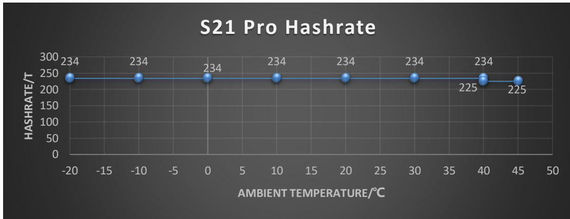
(1) Hashrate vs. Ambient Temperature
